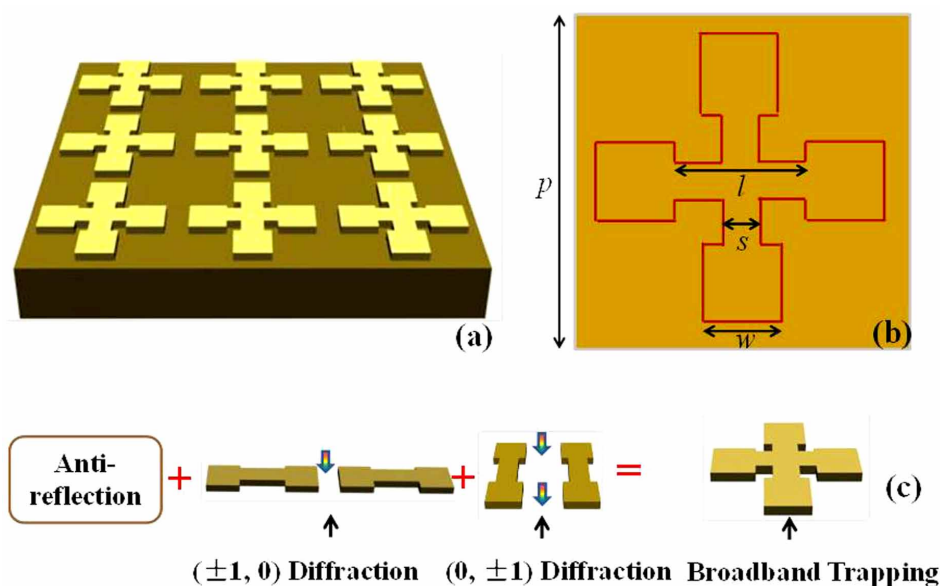
Figure 1 | Schematics illustrating the (a) periodical structure and (b) unit cell of the THz wave absorber. (c) The fundamental principal of THz wave absorption for broadband operation.
